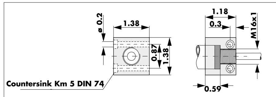
Fixing block
