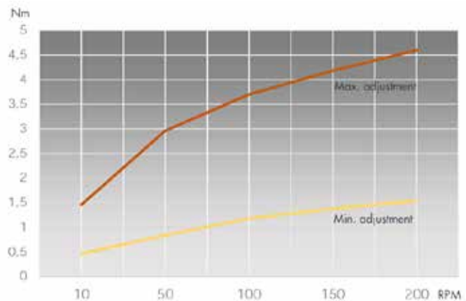
Radial dampers LD 100
