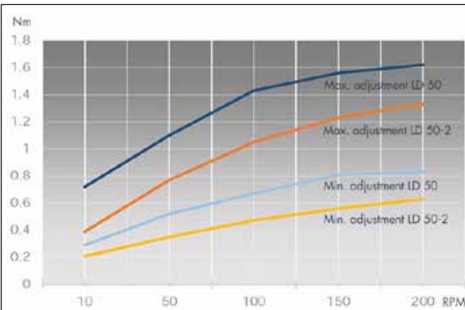
Radial dampers LD 50 / LD 50-2
